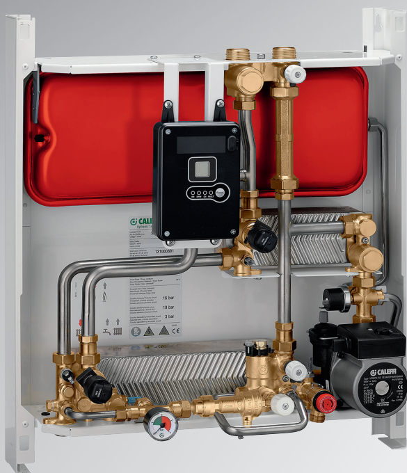
壁挂式-SATK 30
