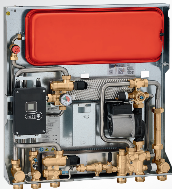
嵌墙式-SATK 60
